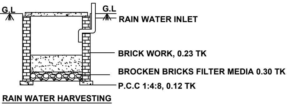
RAIN WATER HARVESTING
