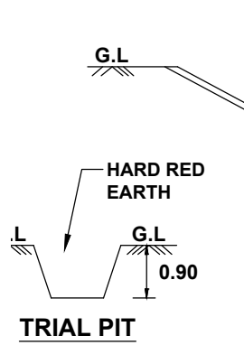
TRIAL PIT
