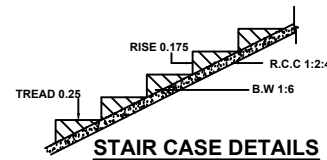
STAIR CASE DETAILS
