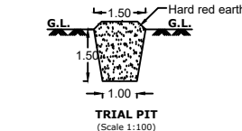
TRIAL PIT (Scale 1:100)
