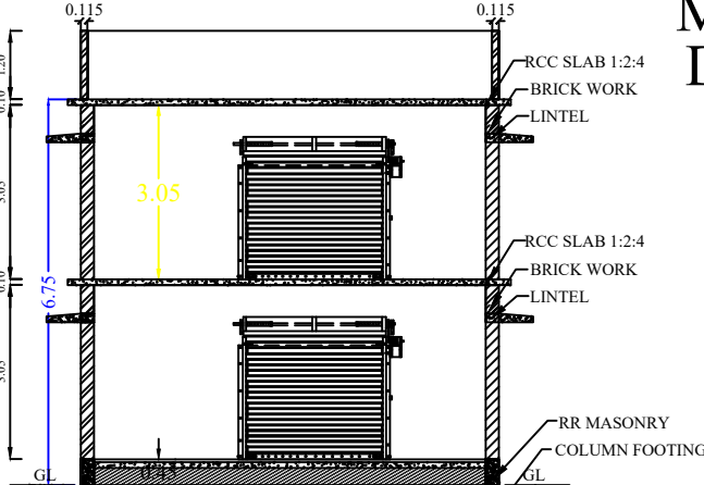
SECTION @ X-X'
