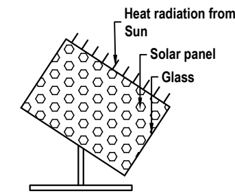
SOLAR SYSTEM
