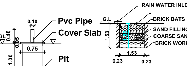
RAIN WATER HARVESTING PIT
