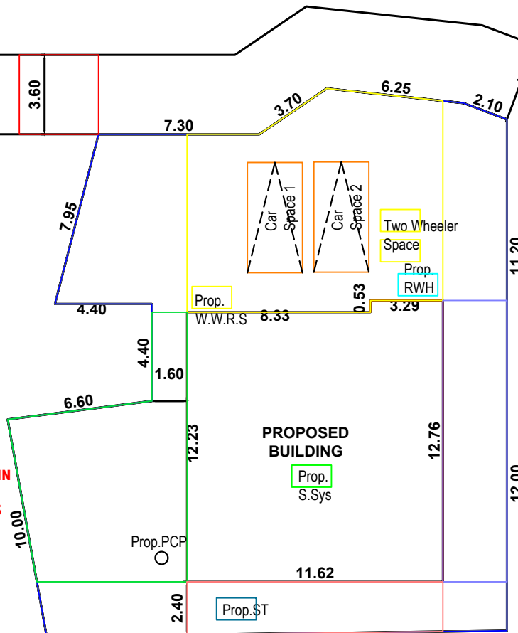
SITE PLAN
