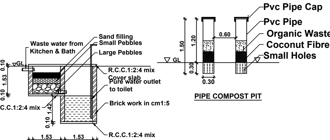
WASTE WATER RECYCLING SYSTEM
