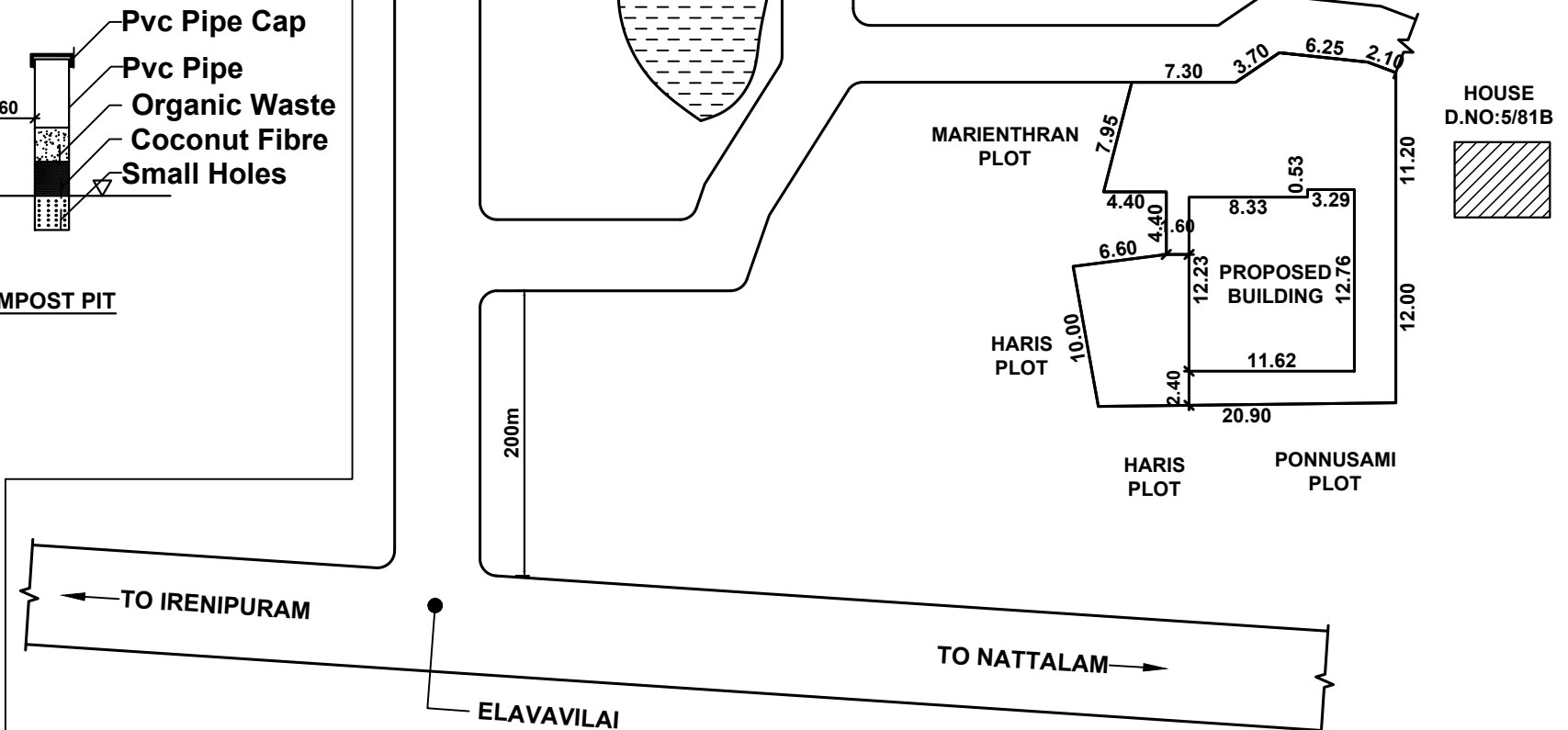
KEY PLAN
