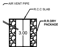
SECTION OF SOAKPIT
