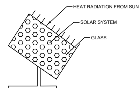
SOLAR SYSTEM
