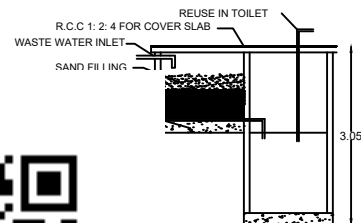
REUSE IN TOILET WASTE WATER INLET SAND FILLING CYCLING OF WASTE WATER
