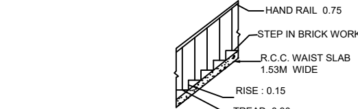
STAIR CASE SECTION
