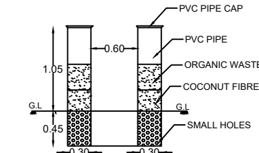
PIPE COMPOSIT PIT
