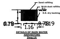
DETAILS OF RAIN WATER HARVESTING DIAGRAM
