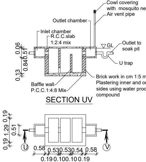
SEPTIC TANK PLAN
