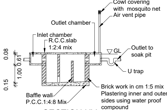
SECTION UV
