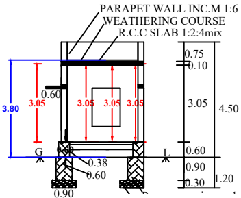
SECTION ON
