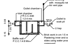
SECTION UV
