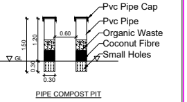
PIPE COMPOST PIT
