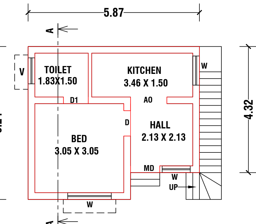
GROUND FLOOR PLAN SCALE 1:100 ALL DIMENSIONS ARE IN "METER"
