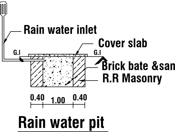
Rain water pit
