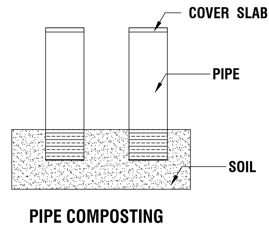
PIPE COMPOSTING
