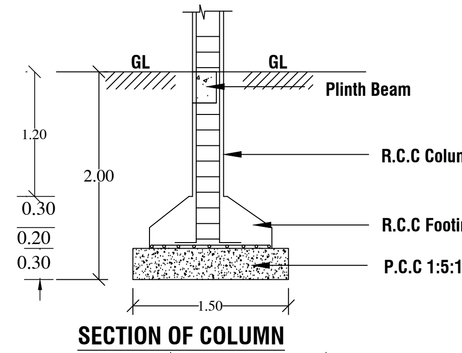
SECTION OF COLUMN
