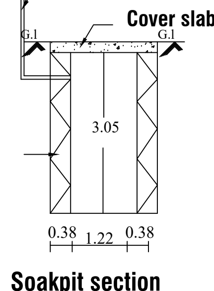
Soakpit section
