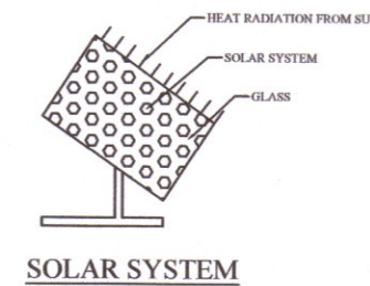
SOLAR SYSTEM
