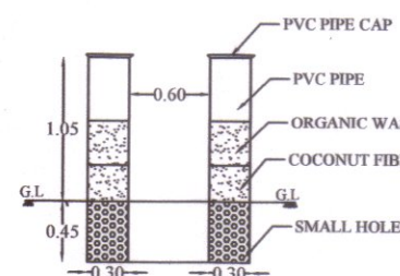
PIPE COMPOSIT PIT
