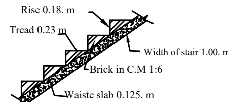
Stair Details
