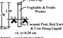
PIPE COMPOSTER
