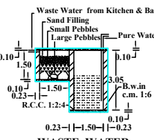
WASTE WATER RECYCLING SYSTEM
