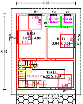
PLAN (FIRST FLOOR)
