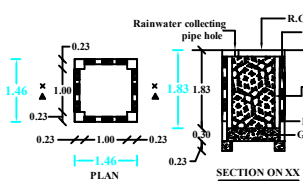
RAIN WATER HARVEST WELL
