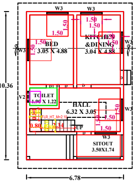
PLAN (GROUND FLOOR)
