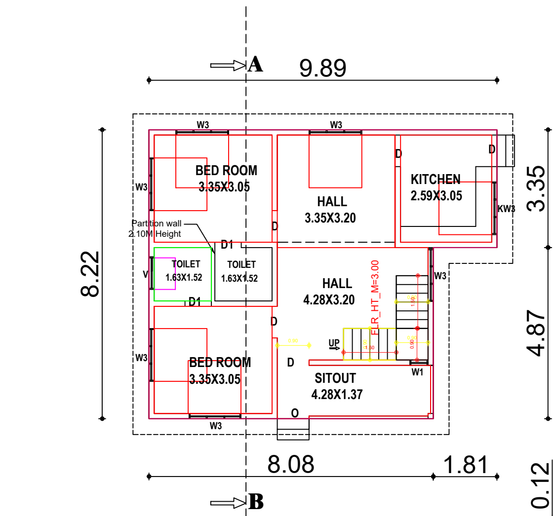
SCALE 1:100 GROUND FLOOR- PLAN ALL DIMENSIONS ARE IN METRE
