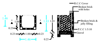
RAIN WATER HARVEST WELL
