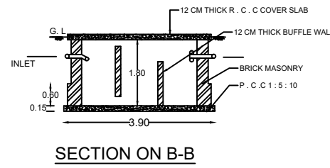
SECTION ON B-B
