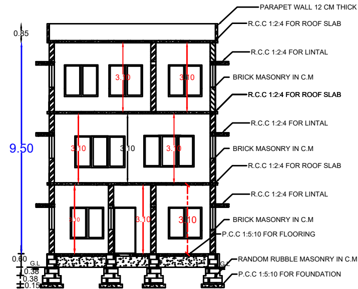
SECTION
