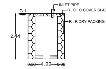
RAIN WATER STORAGE TANK SECTION
