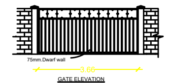
GATE ELEVATION
