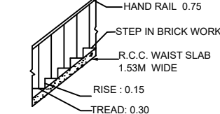
STAIR CASE SECTION
