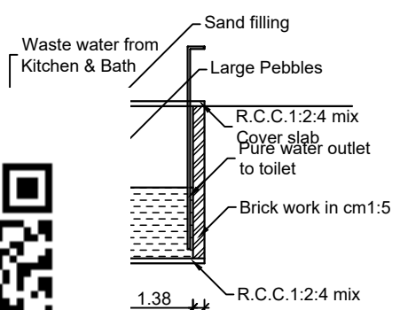
RECYCLING SYSTEM
