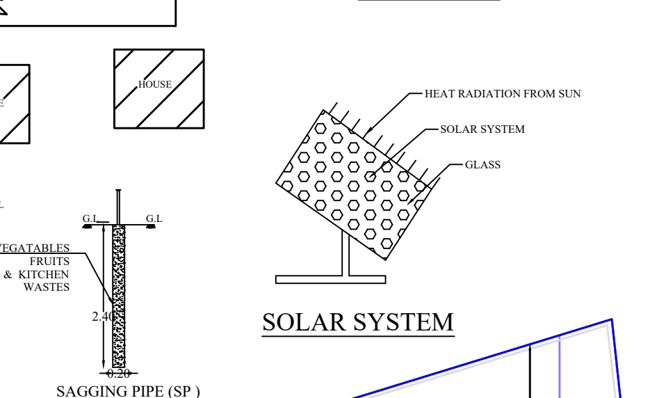
TOPO PLAN (NOT TO SCALE)
