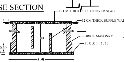
SECTION ON B-B
