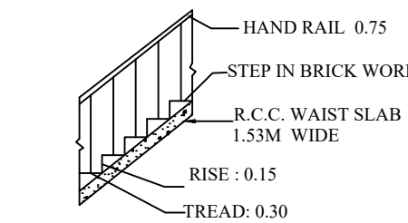
STAIR CASE SECTION
