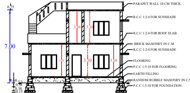
SECTION
