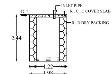
RAIN WATER STORAGE TANK SECTION
