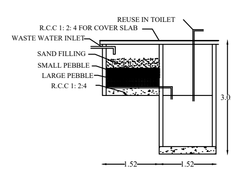
RECYCLING OF WASTE WATER
