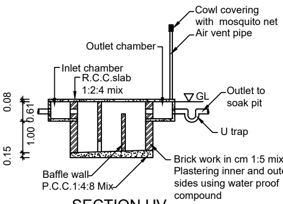
SECTION UV
