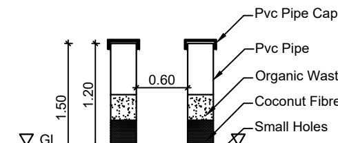
PIPE COMPOST PIT
