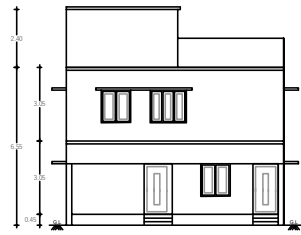
ELEVATION Scale 1:100
