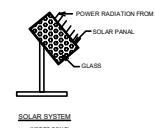
SOLAR SYSTEM
