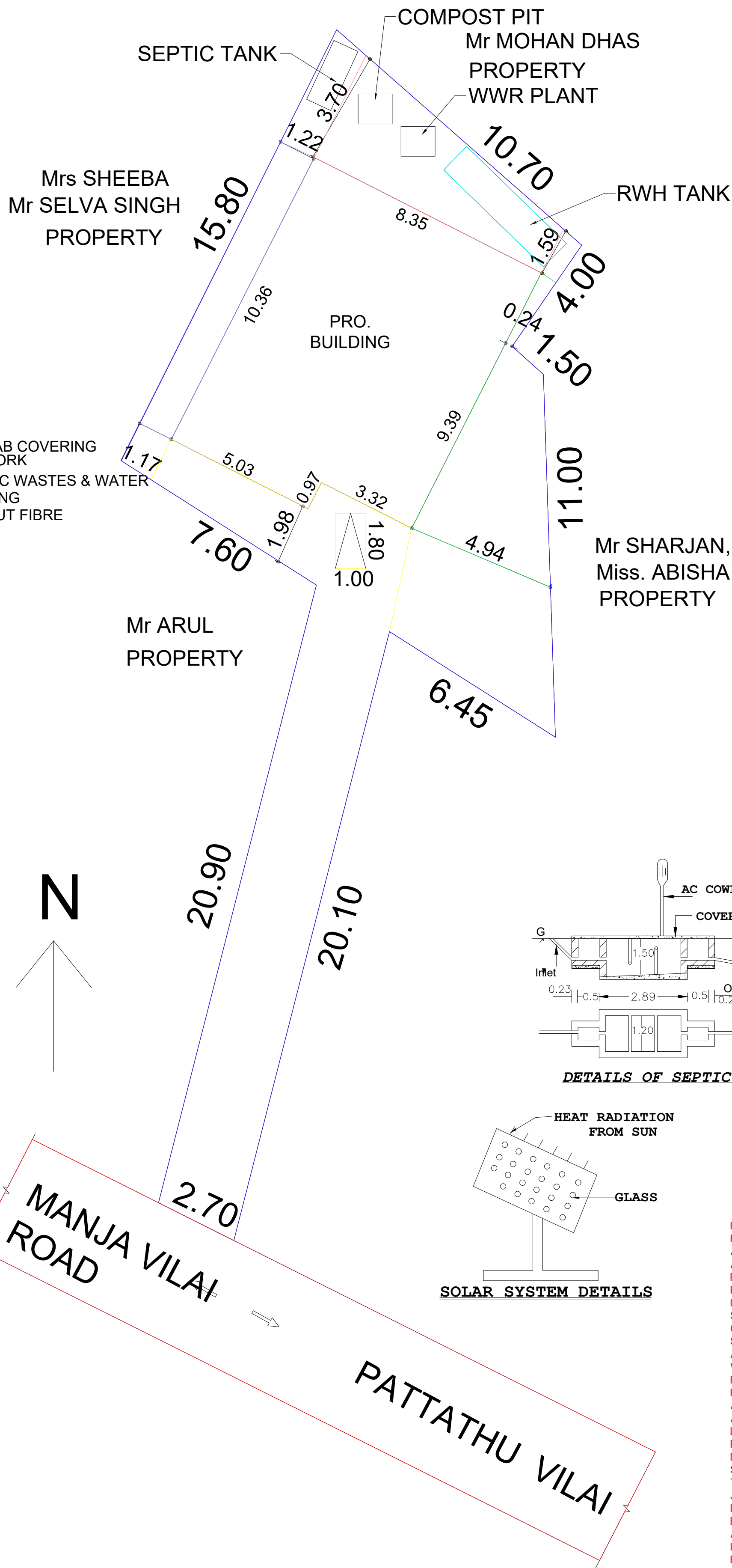
SITE PLAN SCALE 1:100 ALL DIMENSIONS ARE IN METRE
