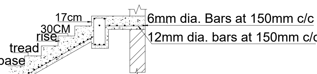
SECTION OF STAIRCASE
