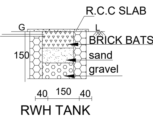
RWH TANK
