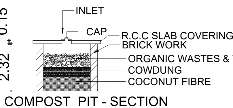
COMPOST PIT - SECTION
