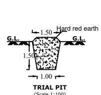
TRIAL PIT (Scale 1:100)
