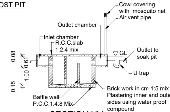
SECTION UV
