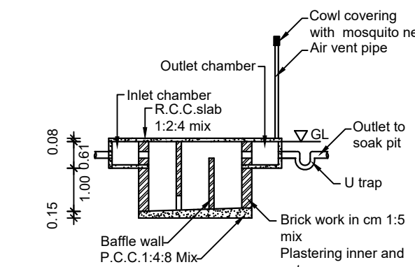
SECTION UV
