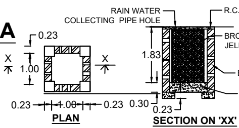
RAIN WATER HARVEST WELL
