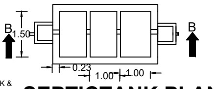
SEPTICTANK PLAN
