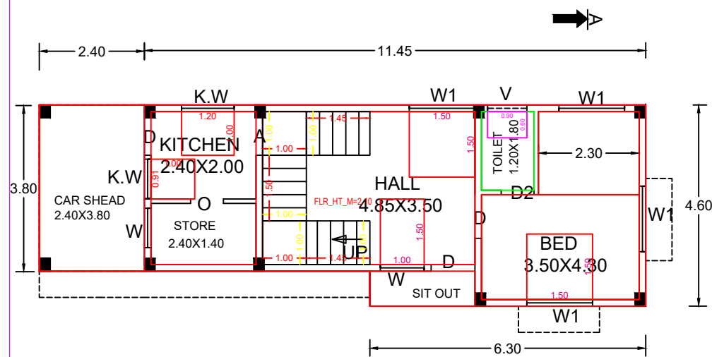
G.F. PLAN
