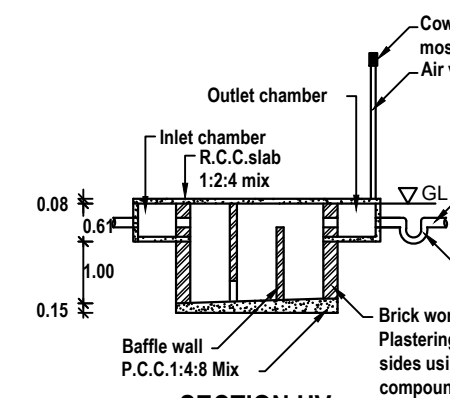
SECTION UV
