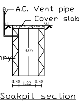
Soakpit section
