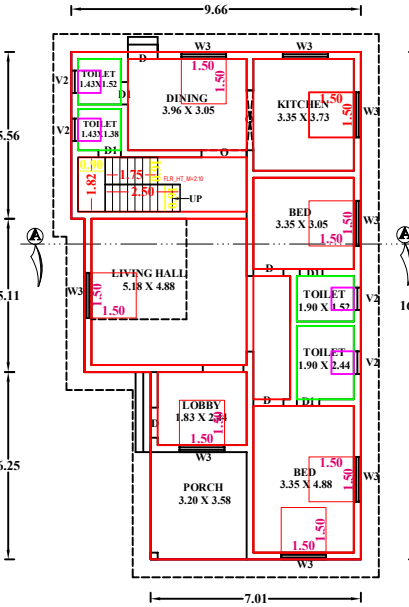
PLAN (GROUND FLOOR)
