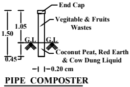
PIPE COMPOSTER
