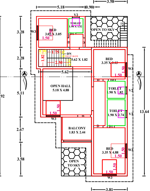
PLAN (FIRST FLOOR)
