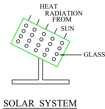
SOLAR SYSTEM
