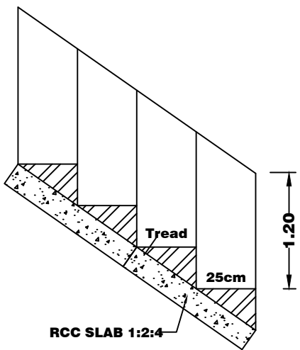
STAIR DETAILS
