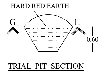
TRIAL PIT SECTION
