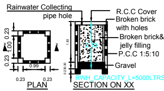
RAIN WATER HARVEST WELL
