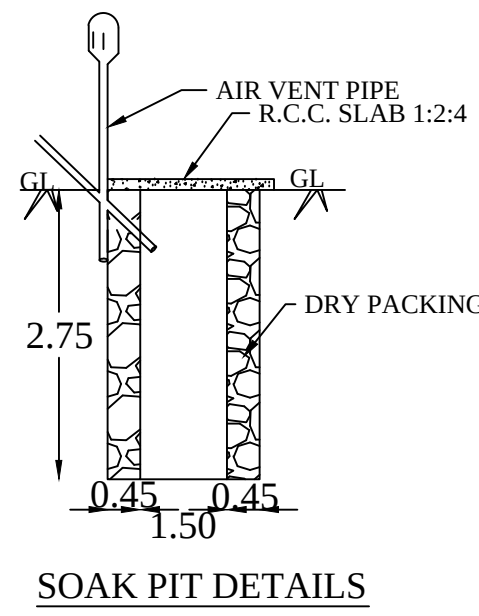
SOAK PIT DETAILS
