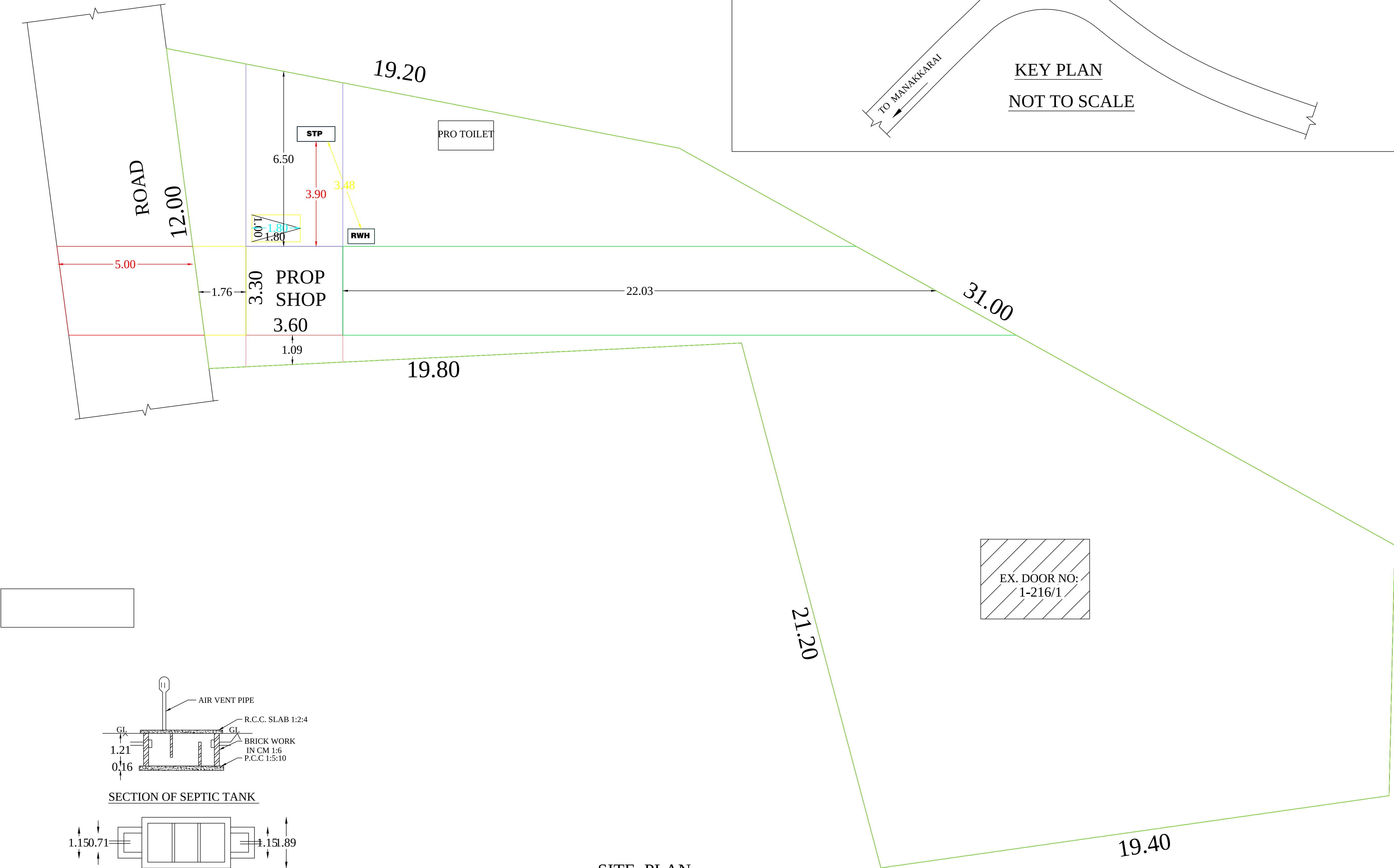
SITE PLAN
