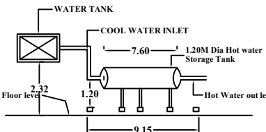
SOLAR WATER HEATING SYSTEM (S.W.H.S.DETAILS)
