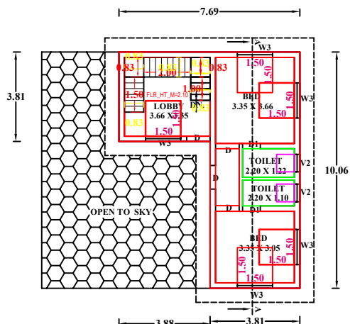
PLAN (FIRST FLOOR)
