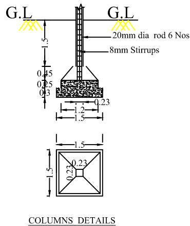
COLUMNS DETAILS
