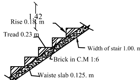
Stair Details
