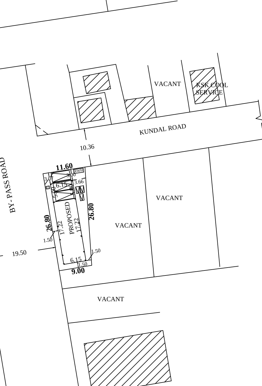
KEY PLAN
