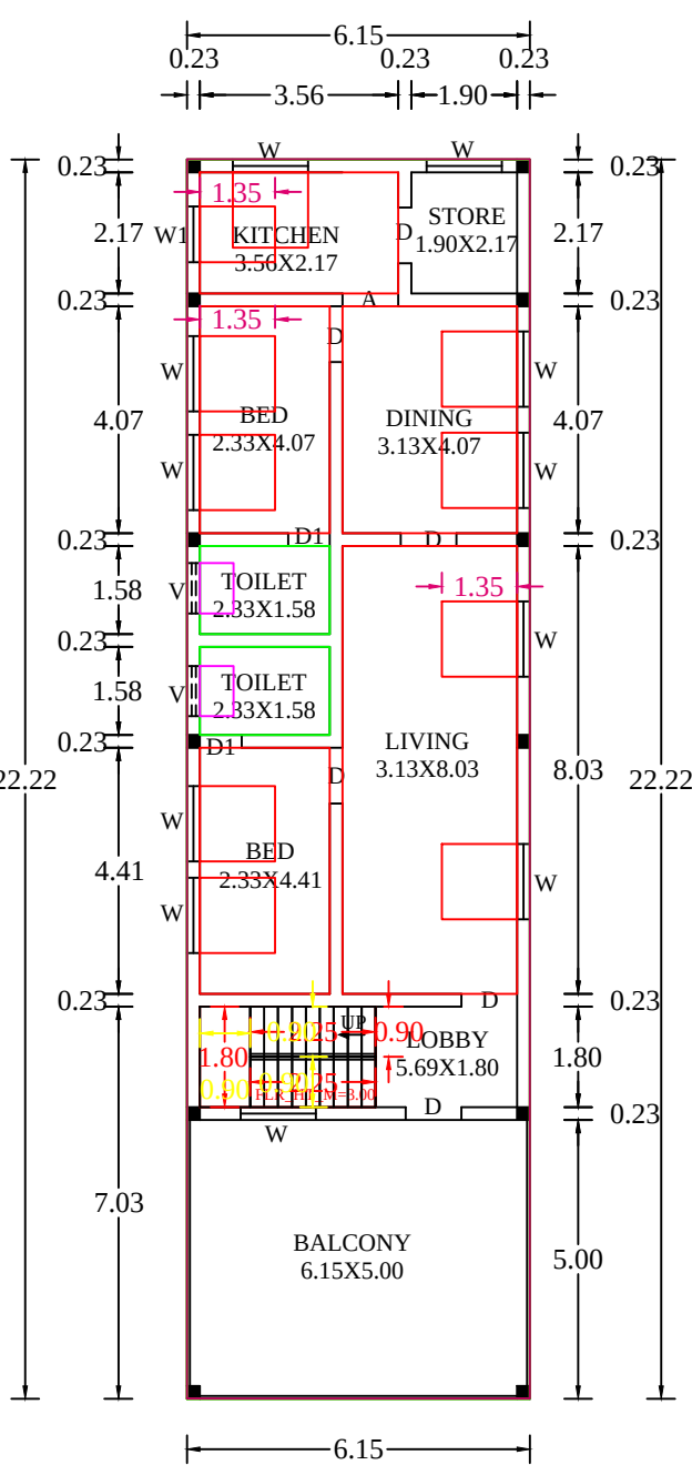
PLAN OF SECOND FLOOR
