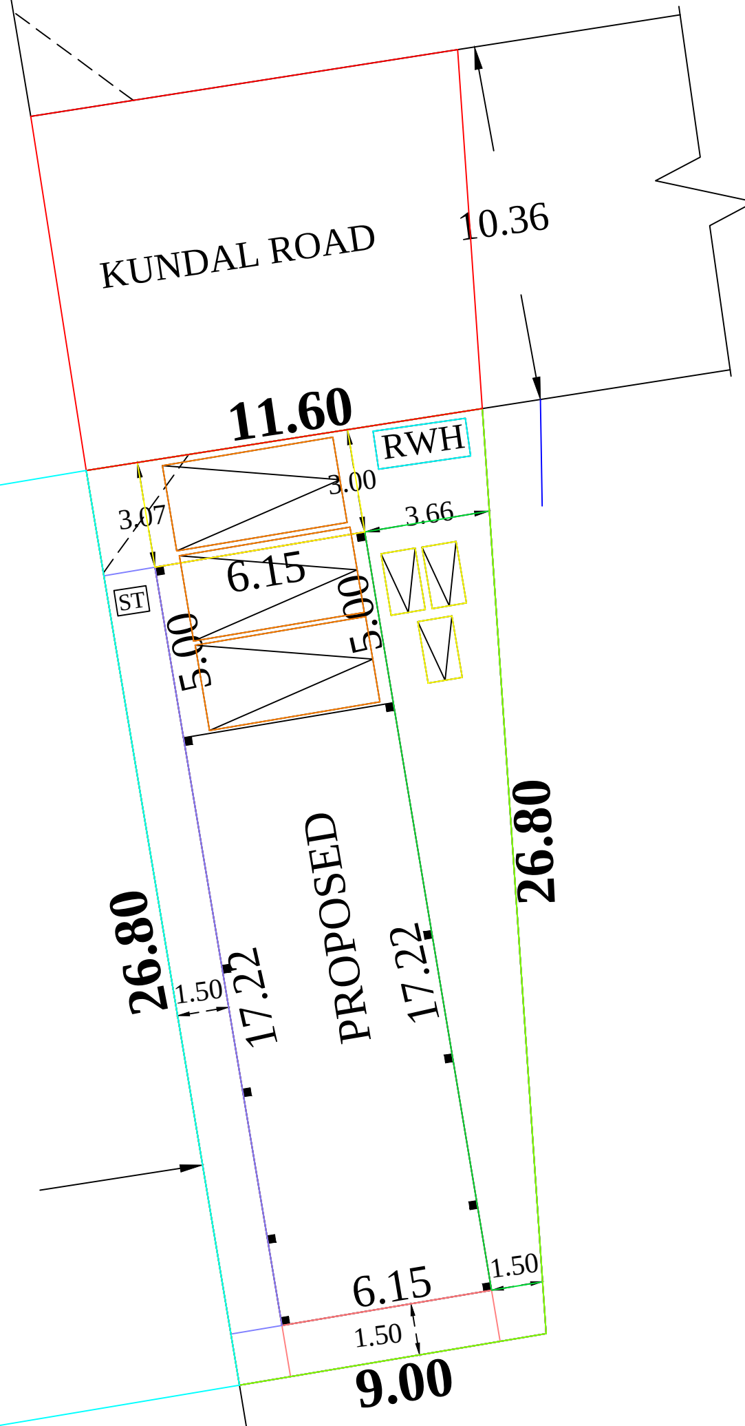
SITE PLAN
