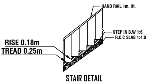
STAIR DETAIL
