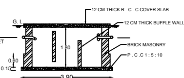
SECTION ON B-B
