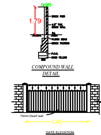
GATE ELEVATION
