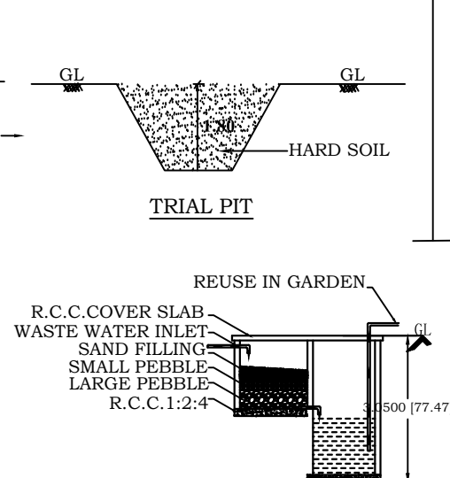
RECYCLING OF WASTE WATER
