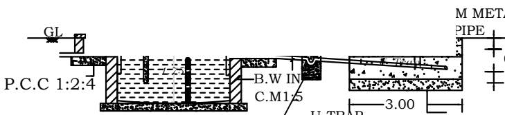
SECTION SECTION OF DISPERSION TRENCH
