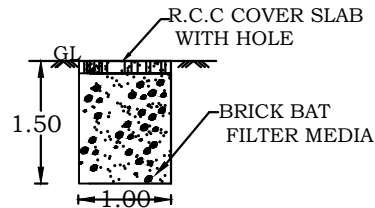
RESTING PIT
