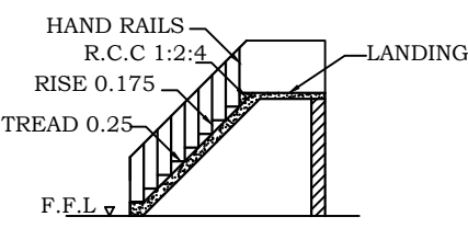
STAIR CASE DETAIL
