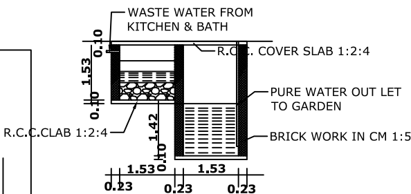
RECYCLING OF WASTE WATER SYSTEM
