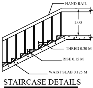
STAIRCASE DETAILS
