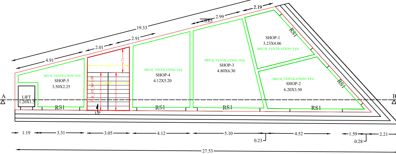
GROUND FLOOR
