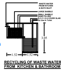
RECYCLING OF WASTE WATER FROM KITCHEN & BATHROOM
