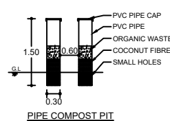
PIPE COMPOST PIT
