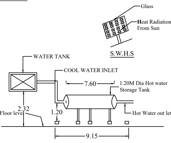
SOLAR WATER HEATING SYSTEM (S.W.H.S.DETAILS)
