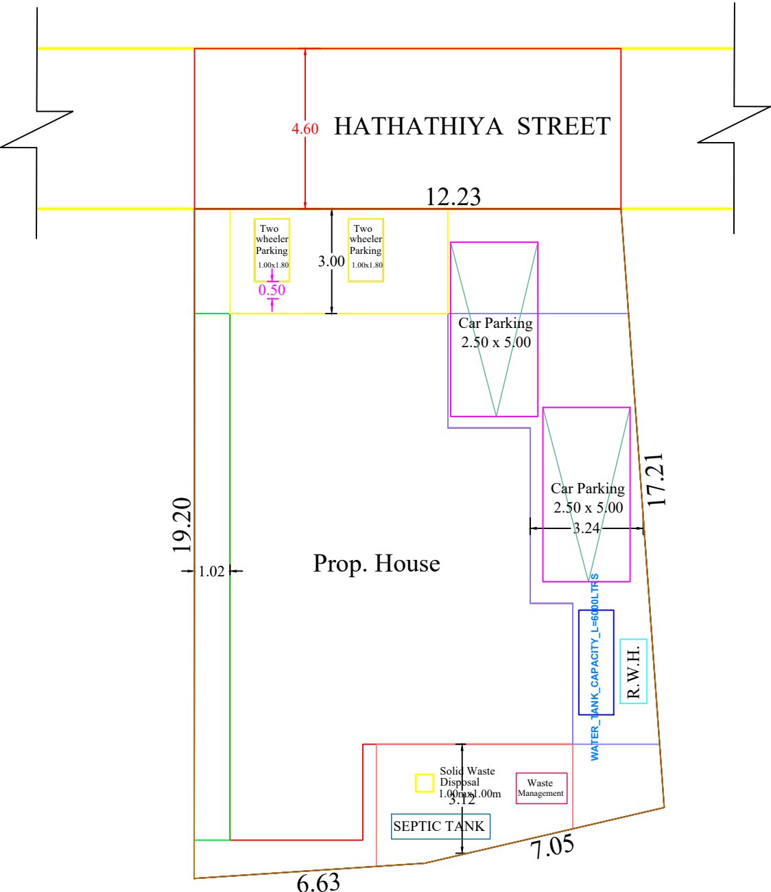
SITE PLAN
