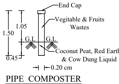
PIPE COMPOSTER
