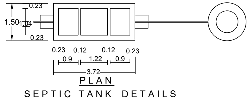
SEPTIC TANK DETAILS
