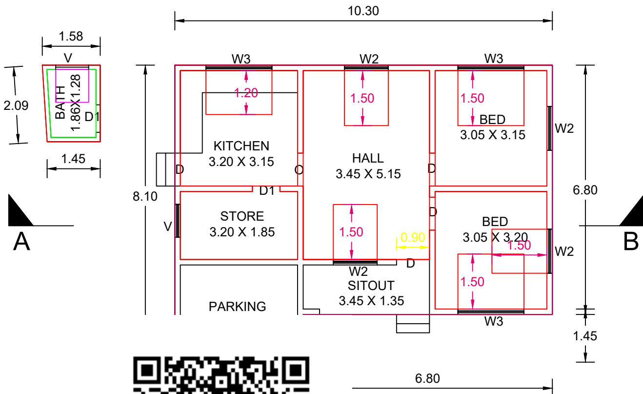
FLOOR PLAN
