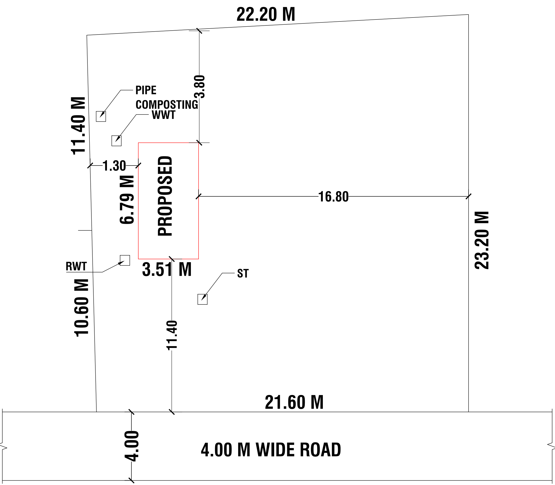
SITE PLAN
