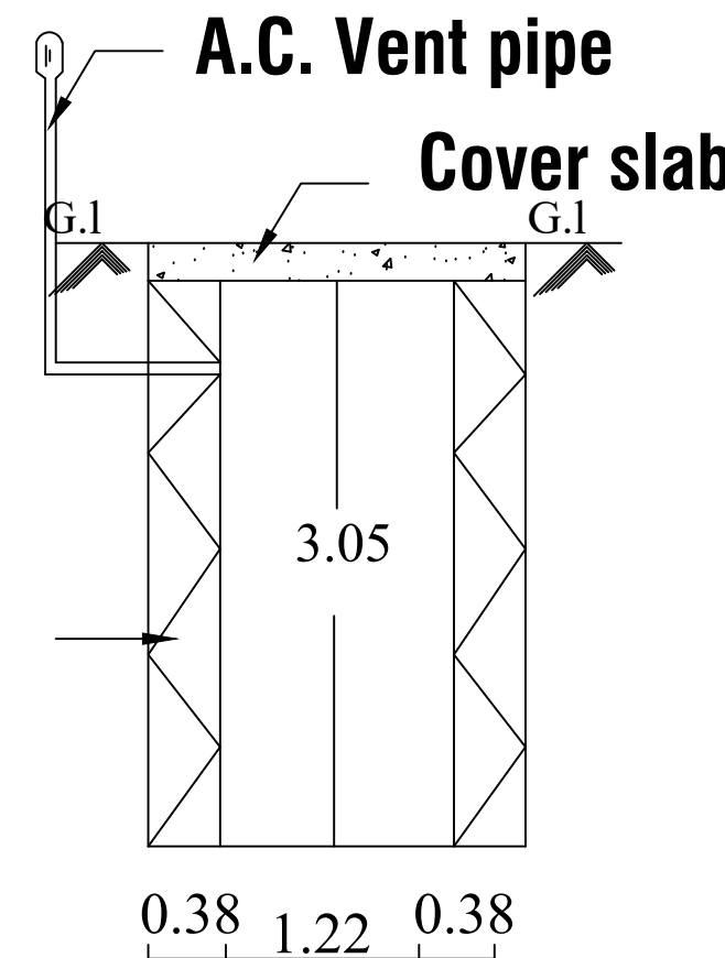
Soakpit section
