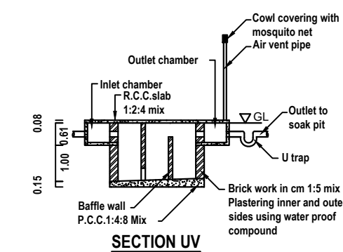
SECTION UV
