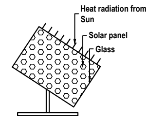
SOLAR SYSTEM
