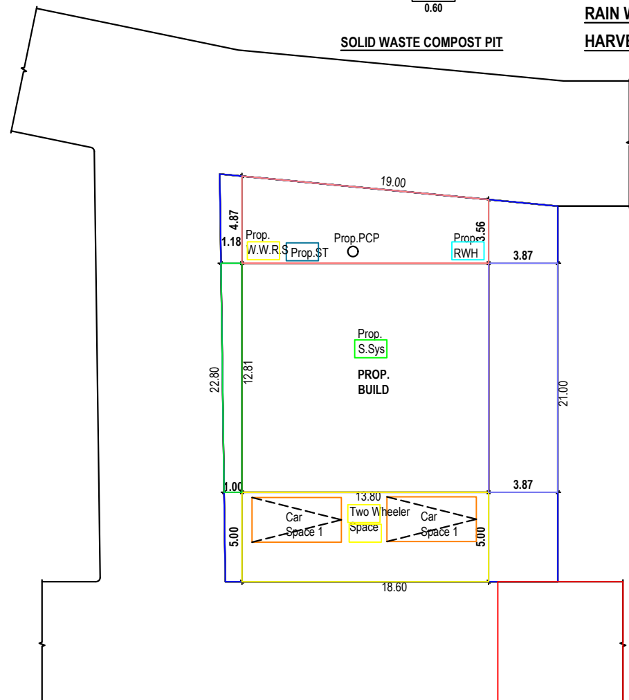
SITE PLAN
