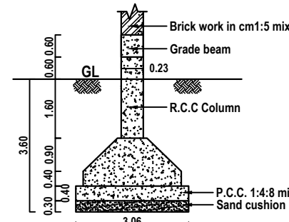
COLUMN DETAILS
