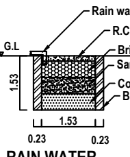
RAIN WATER HARVESTING PIT
