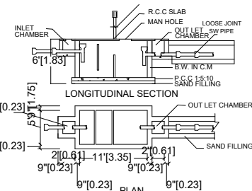
SEPTIC TANK:
