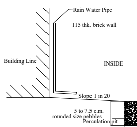
PERCOLATION PIT
