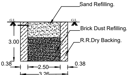
DETAILS OF RAIN WATER HARVESTING Dwg:1A
