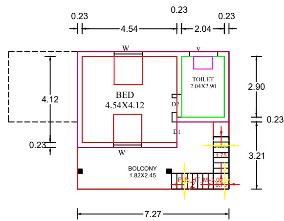
PLAN OF FIRST FLOOR
