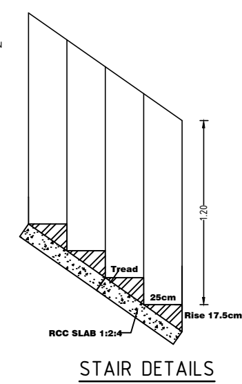
STAIR DETAILS
